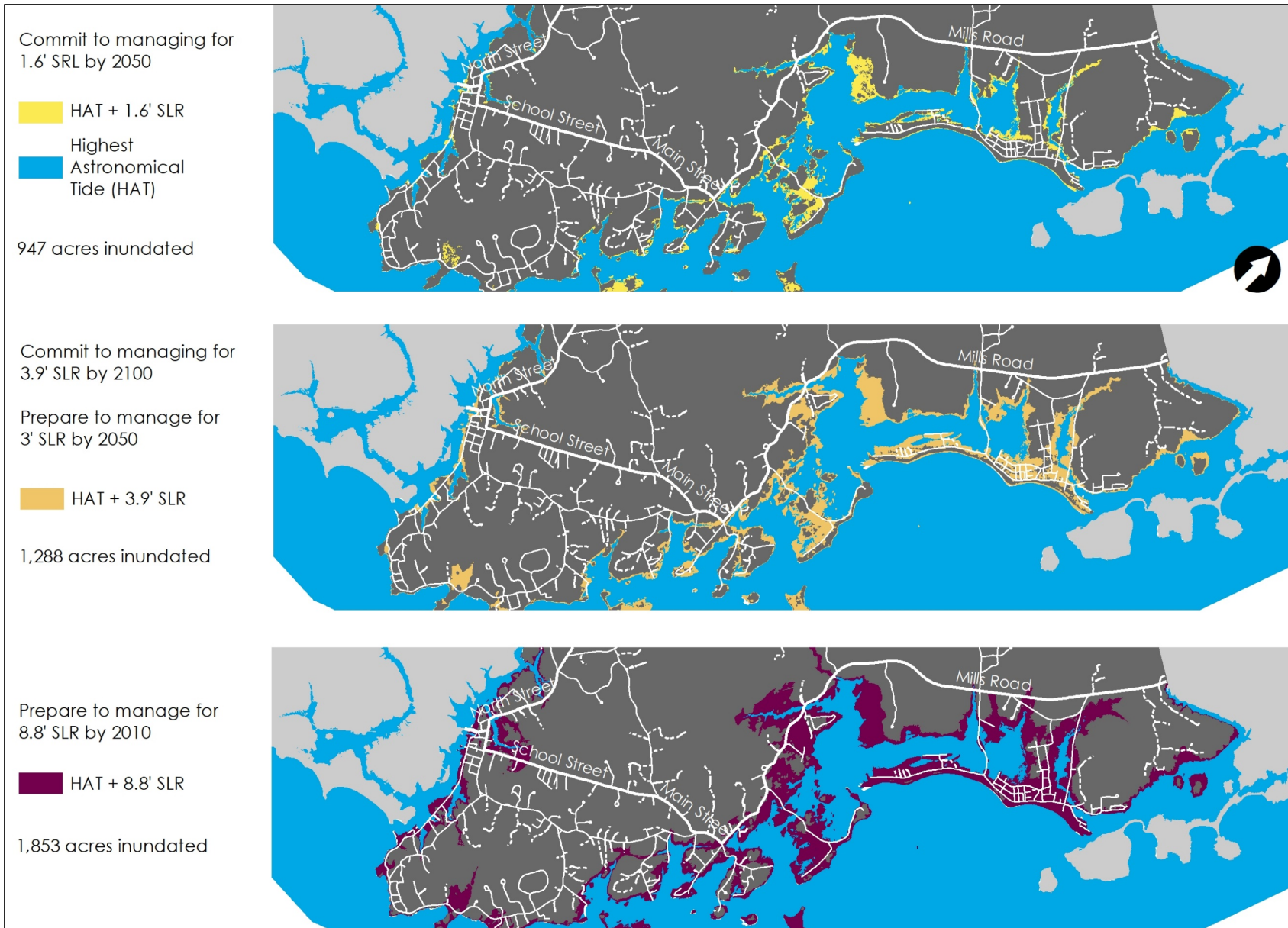
Figure 16-4. Sea level rise and storm surge scenarios (Source: Maine Geological Survey)
