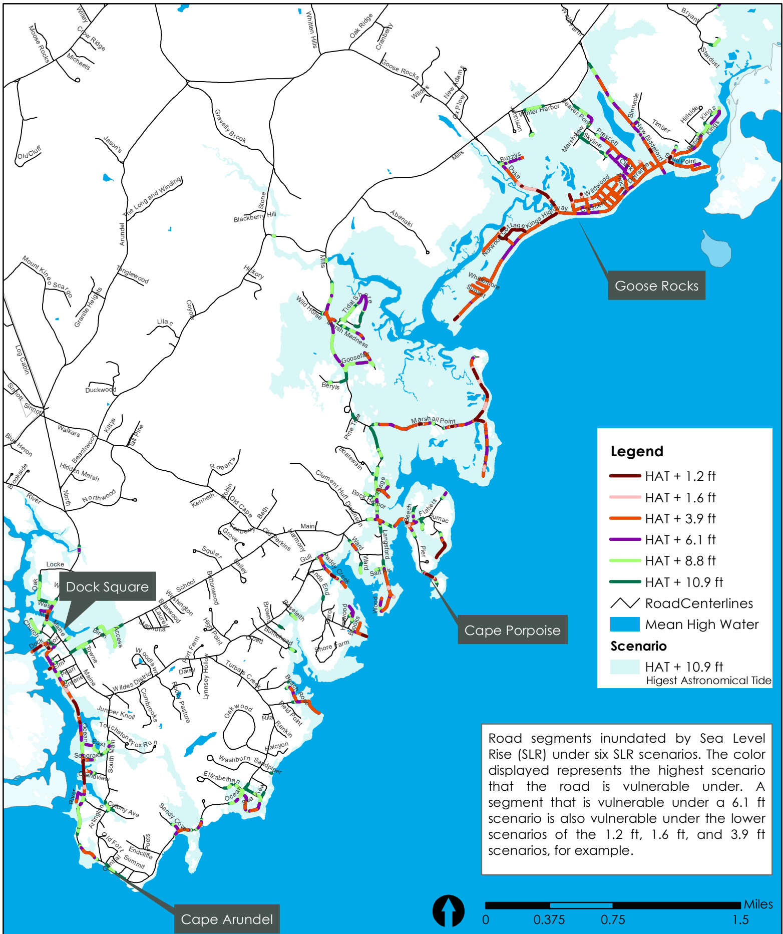
Figure 11-21 Road segments inundated by sea level rise (SLR)
