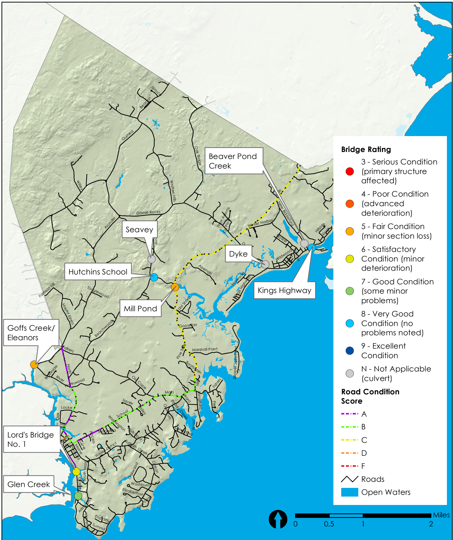
Figure 11-6 Bridges and culverts with bridge and roadway condition
