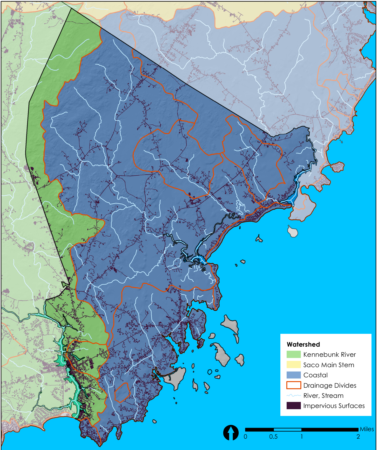
Figure 7-2 Drainage divides
