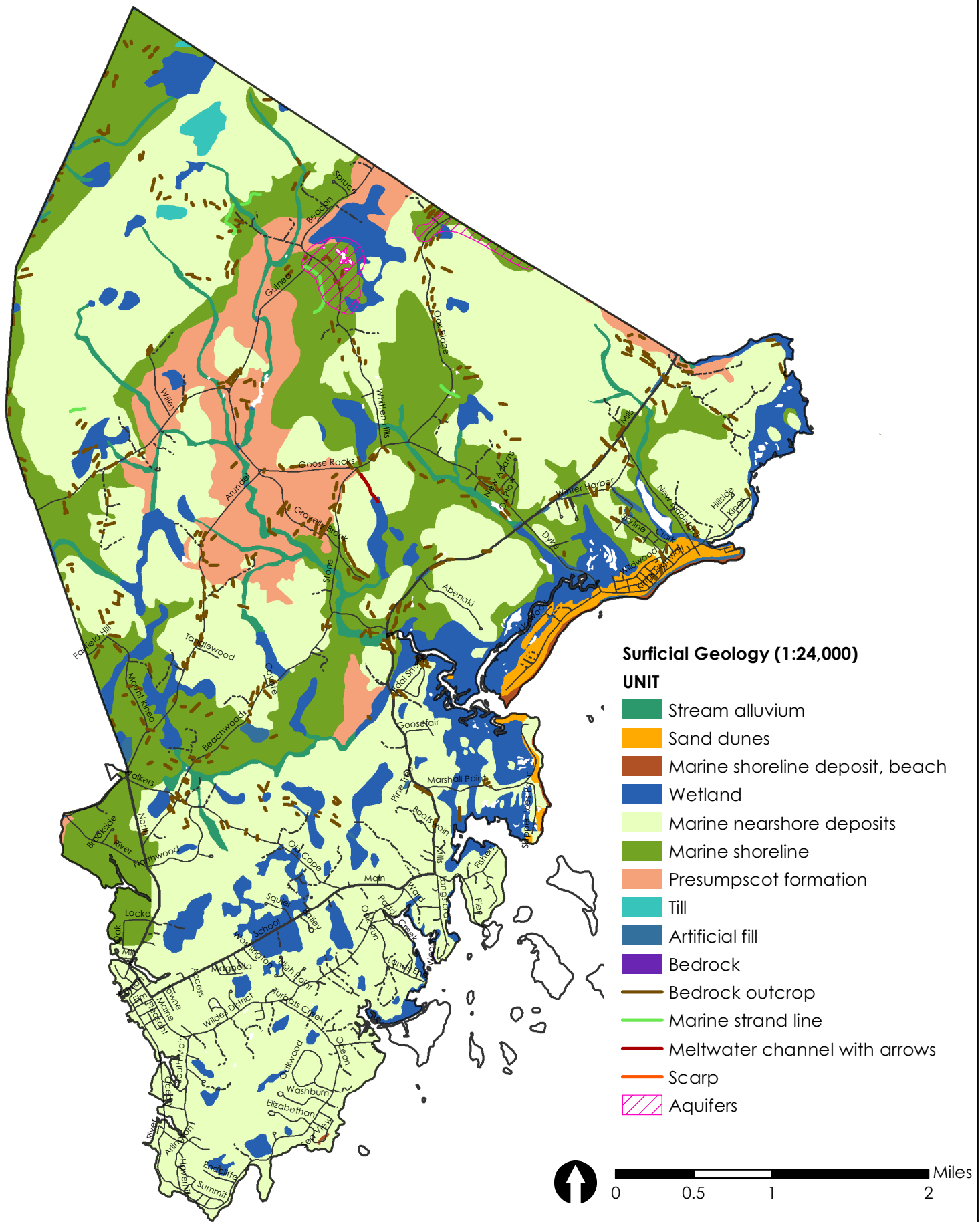
Figure 7-3 Surficial geology and aquifers
