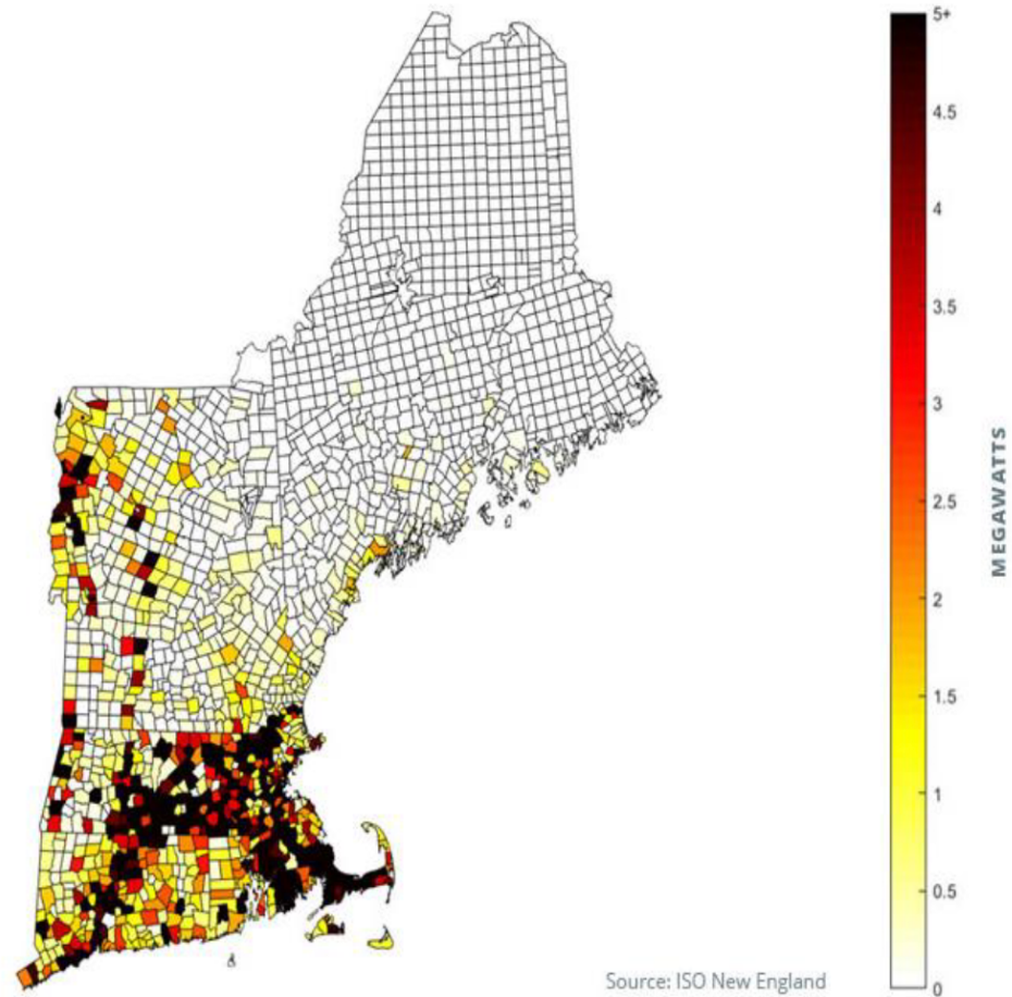
Figure 10-15 Installed Behind-the-Meter Solar Power by Town (Source: ISO New England)
