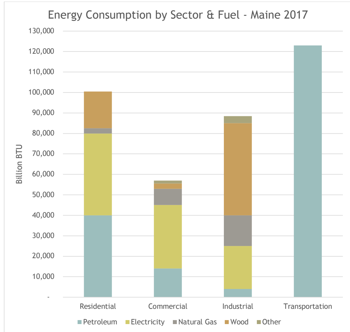
Figure 10-3 Maine Energy Consumption by Sector & Fuel 2017 (Source: EIA, SEDS database)
